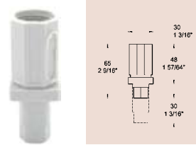
E.3030.PPG 30mm Insert, polypropylene
