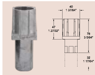
55 303 4000 40mm Insert, bullet/hex 55 303 4001 40mm Insert, bullet/hex, nickel plated
