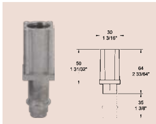
55 303 2000 30mm Insert, bullet/hex
