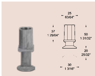
55 303 2500 25mm Insert 55 303 2501 25mm Insert, nickel plated
