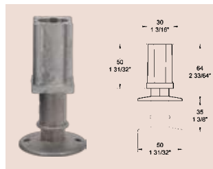
55 303 1000 30mm Insert, flange
