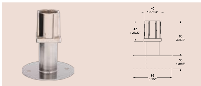
55 303 4004 40mm Insert, flange, nickel plated, stainless steel foot
